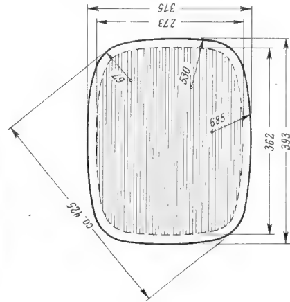
Frontplatte
